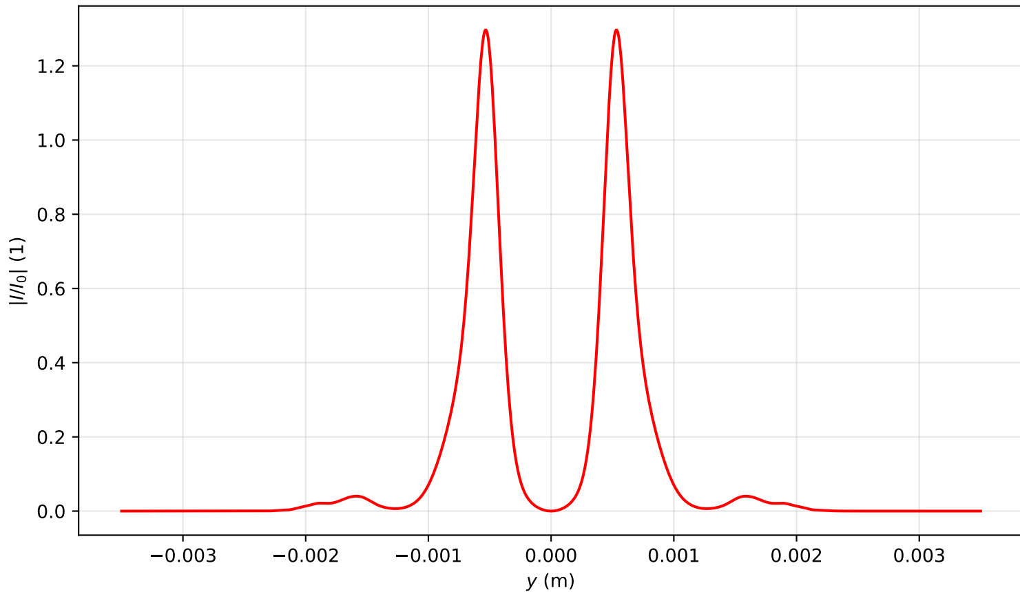
Intensity profile I(x=0, y, z=1.513)/I_0 , P_{in}=8.0P_{cr} , artificial time
